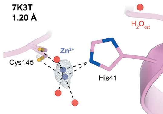
Figure 2 7k3t anomalous density map, contoured at 4\sigma . Anomalous density is only present in the asymmetric unit above 4\sigma in the vicinity of the active site (as shown here). Both Zn^{2+} alternate conformations modeled in 7k3t display tetrahedral coordination geometry, as shown with black dotted lines.
